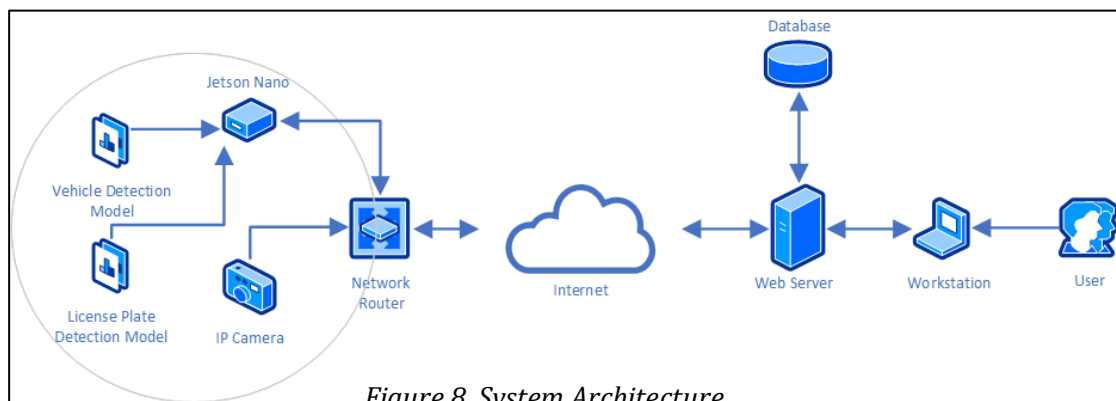
Figure 8. System Architecture
